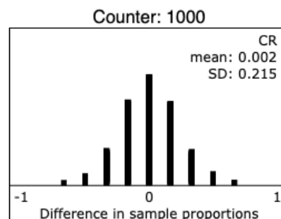
Figure 4: Screenshot from the Randomizing Subjects Applet.
