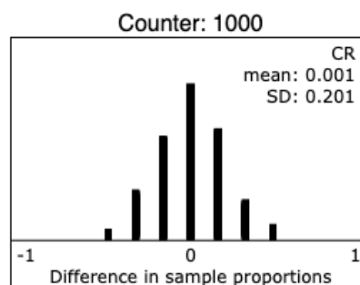
Figure 2: Screenshot from the Randomizing Subjects Applet.
