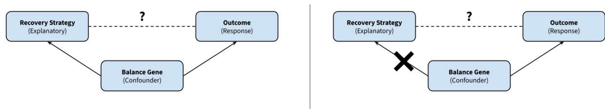
Figure 6: Illustration of the removal of confounders.
