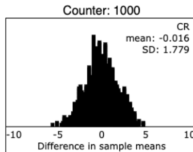
Figure 3: Screenshot from the Randomizing Subjects Applet.
