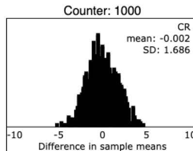
Figure 5: Screenshot from the Randomizing Subjects Applet.
